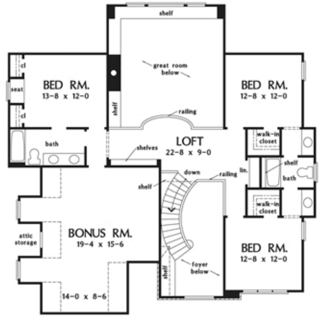
SECOND FLOOR PLAN PLAN NO. 1241
